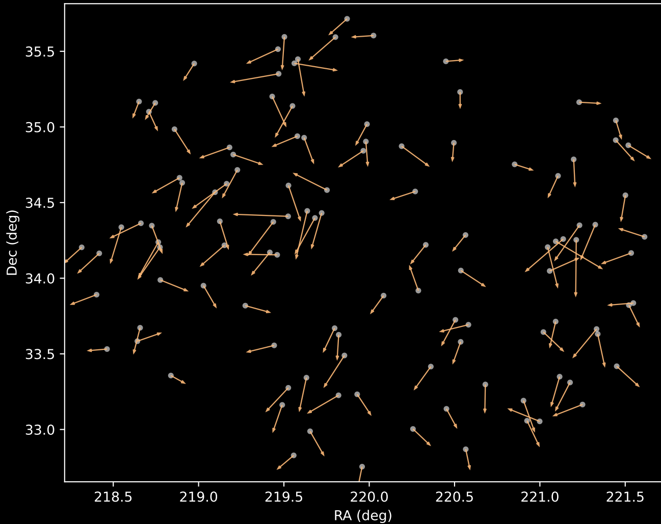
APOGEE DR17 Cluster 3 Proper Motion Vectors (n=113)
