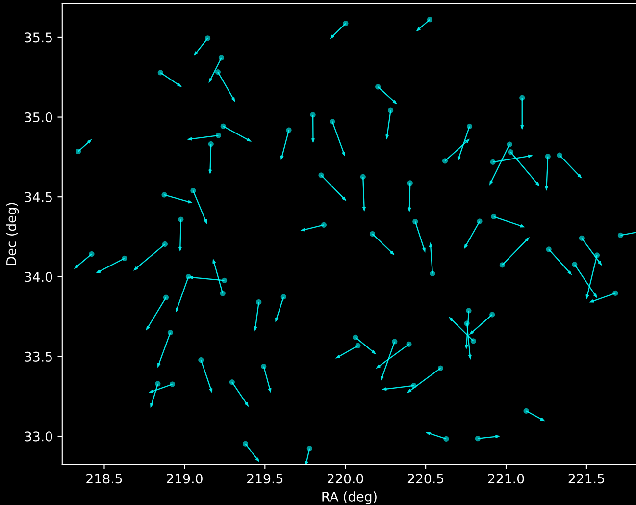
APOGEE DR17 Noise Stream Proper Motion Vectors (n=72)
