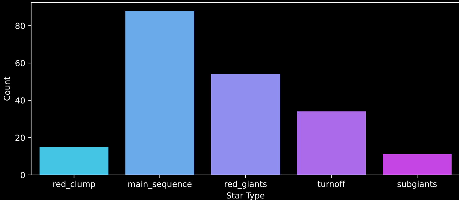
APOGEE DR17 Field: [187+28_MGA] Count plot of Star Type
