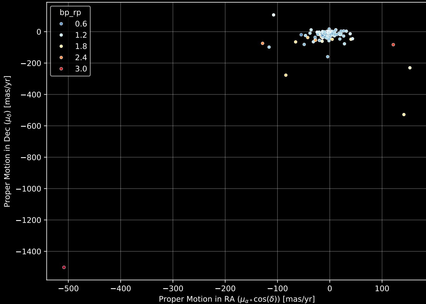
APOGEE DR17 Field: [187+28_MGA] Proper Motion Diagram (n= 202)
