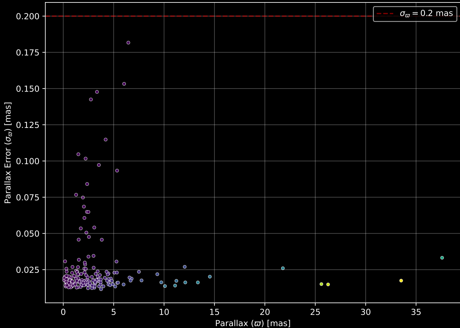
APOGEE DR17 Field: [187+28_MGA] Parallax Quality (n= 202)
