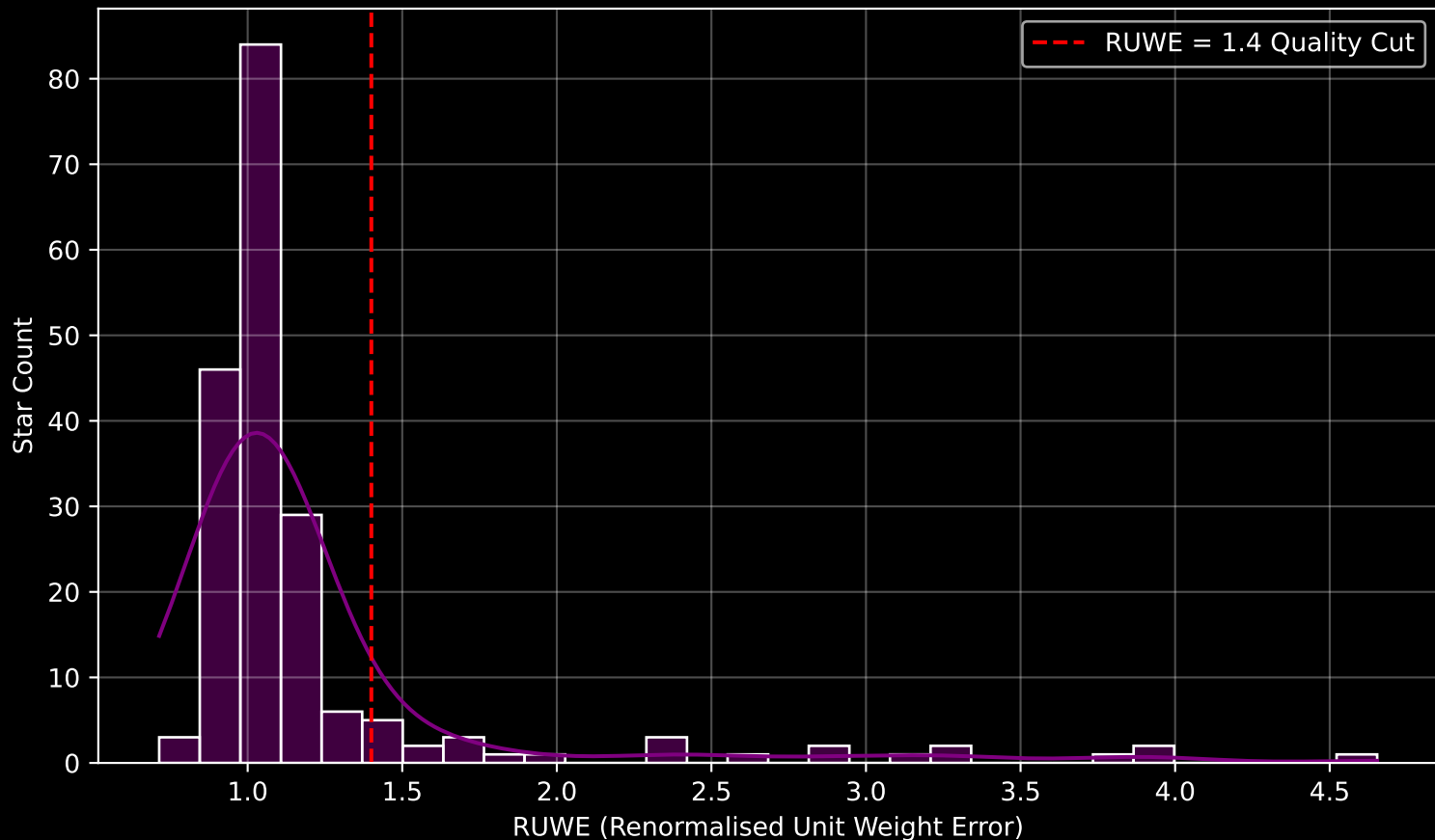
GAPOGEE DR17 Field [187+28_MGA] RUWE Distribution (n= 193)
