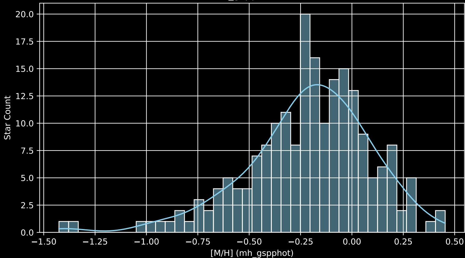
APOGEE DR17 Field: [187+28_MGA [M/H] (mh_gspphot) (n= 201)
