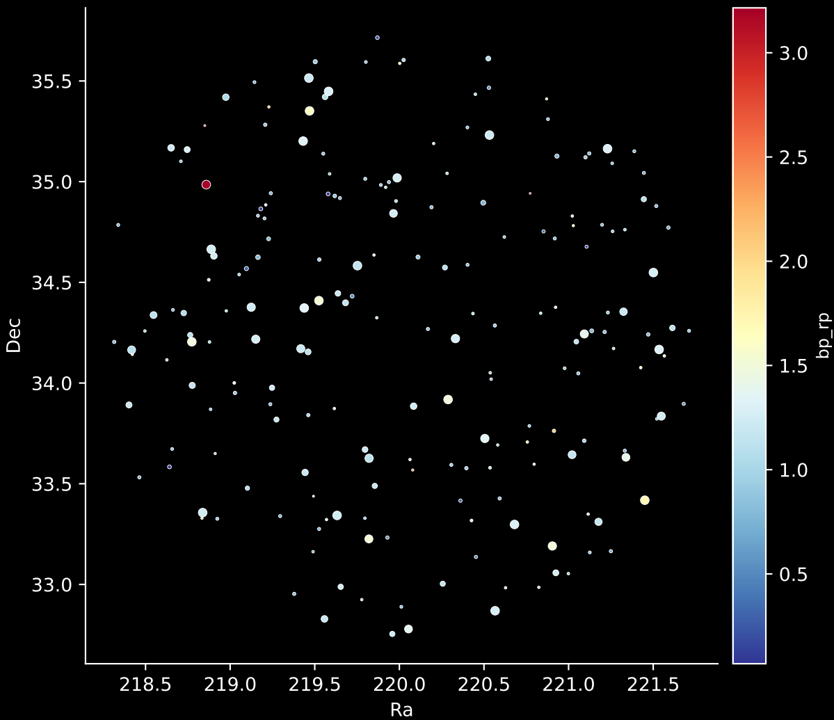
APOGEE DR17 Field: [187+28_MGA] Stars: 202
